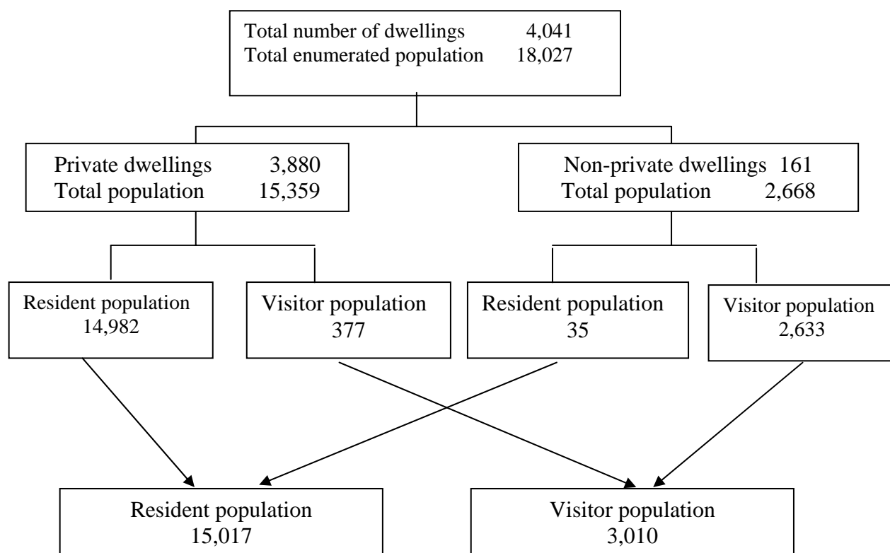
Figure 2: Population composition
