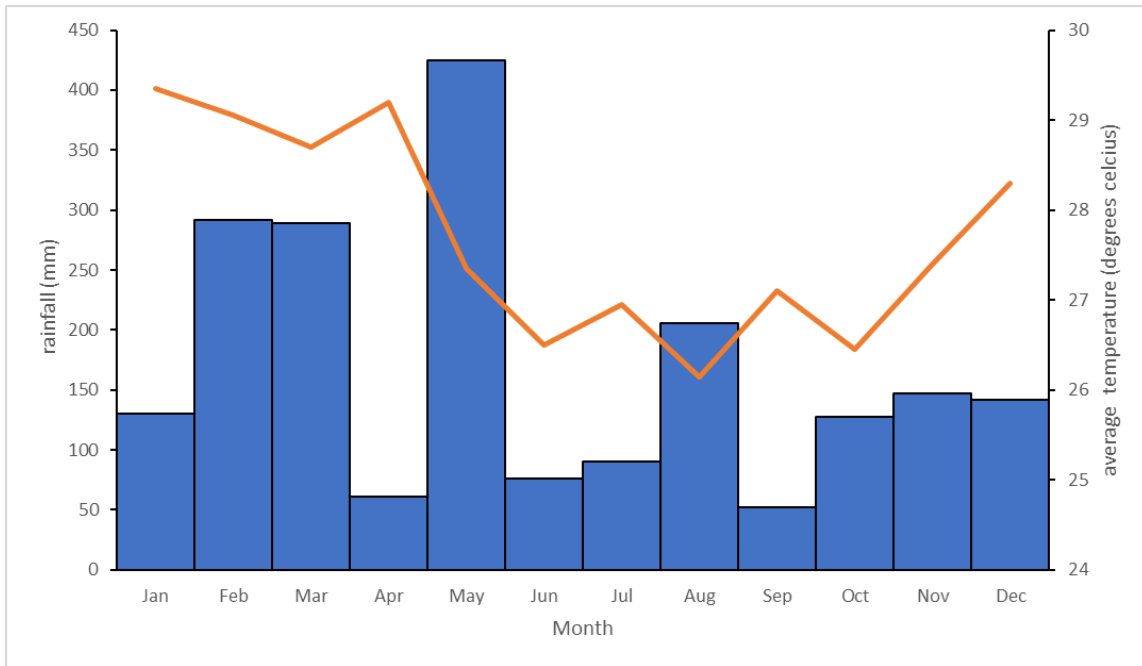
Figure 4: Palmerston Atoll AWS data for 2021
