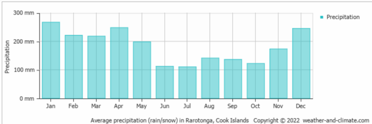
Figure 5: Average precipitation in Rarotonga, Cook Islands
